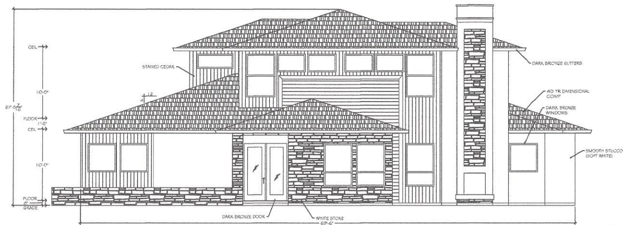
1 9 FRONT ELEVATION SCALE 1/4" = 1'-0"
